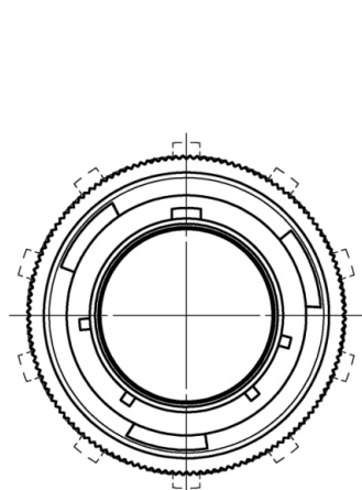
Style 06T/06TG/06E/06EG Style 46T/46TG/46E/46EG (dashed line) Front view
